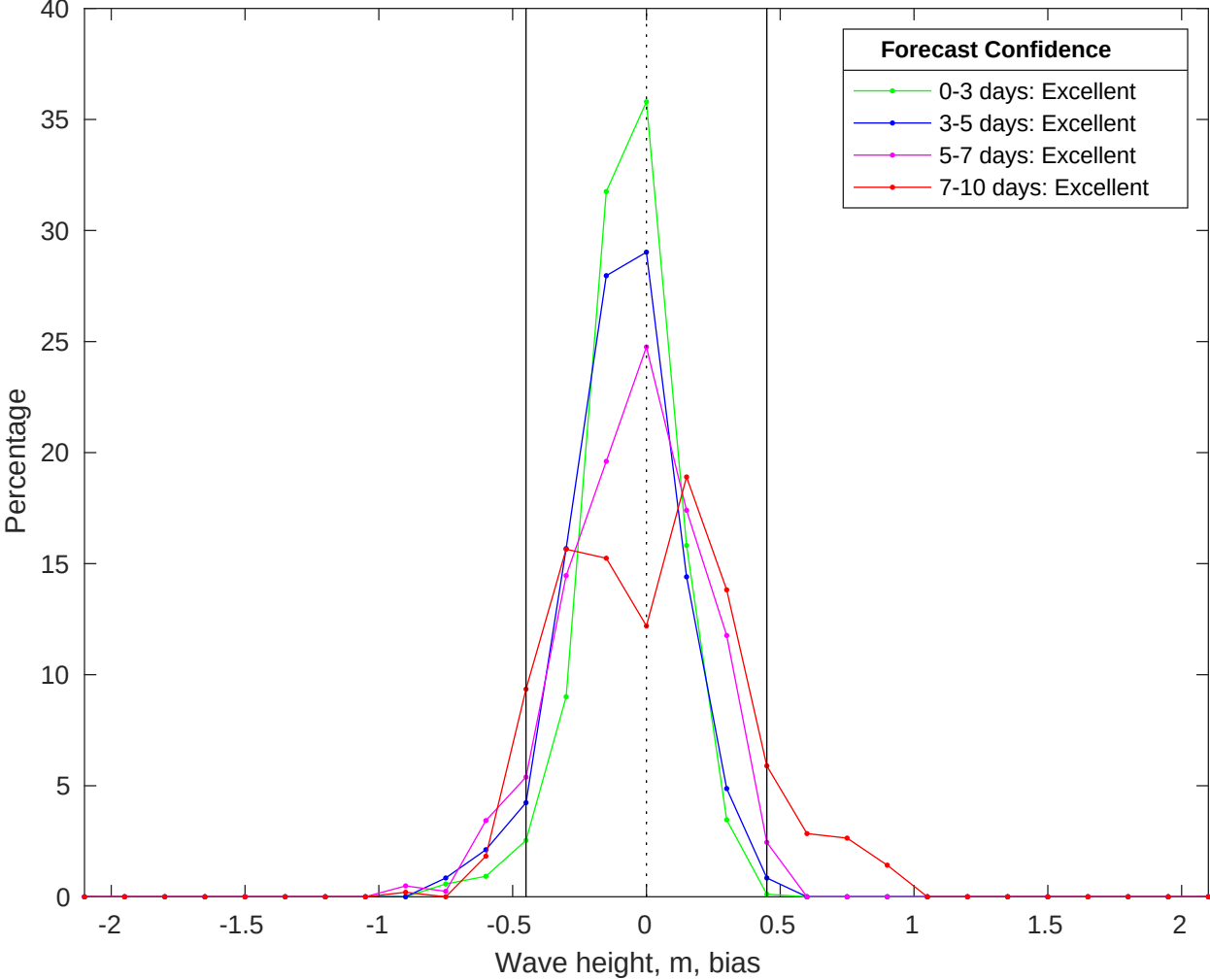
NDBC 46215 vs CMEMS Waves Bias Histogram: 24-Oct-2025
