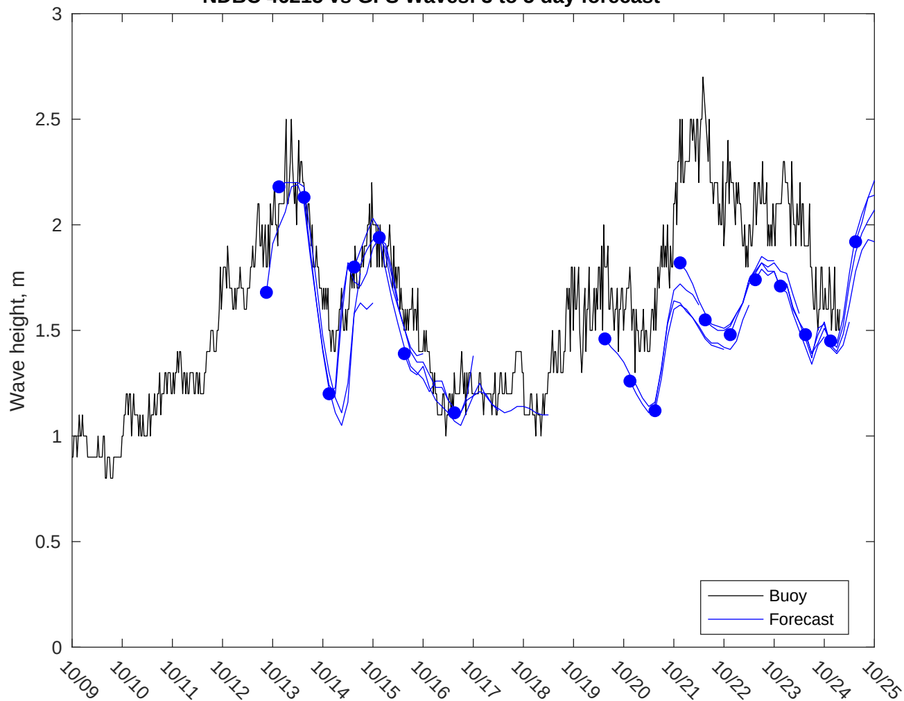
NDBC 46215 vs GFS Waves: 3 to 5 day forecast
