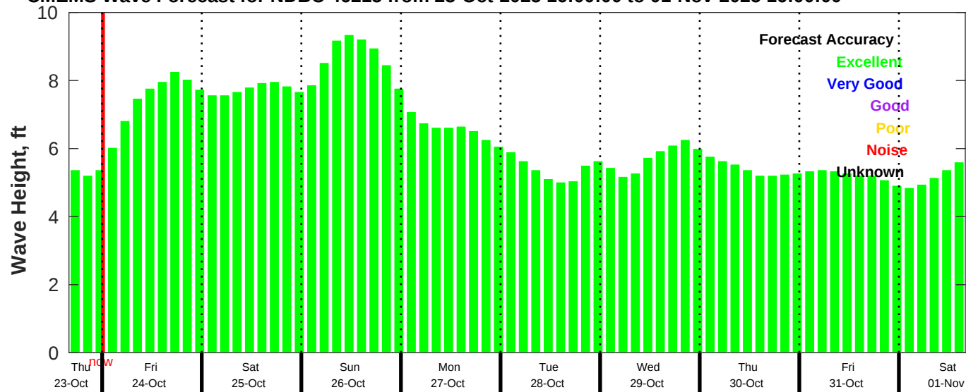
CMEMS Wave Forecast for NDBC 46215 from 23-Oct-2025 16:00:00 to 01-Nov-2025 16:00:00
