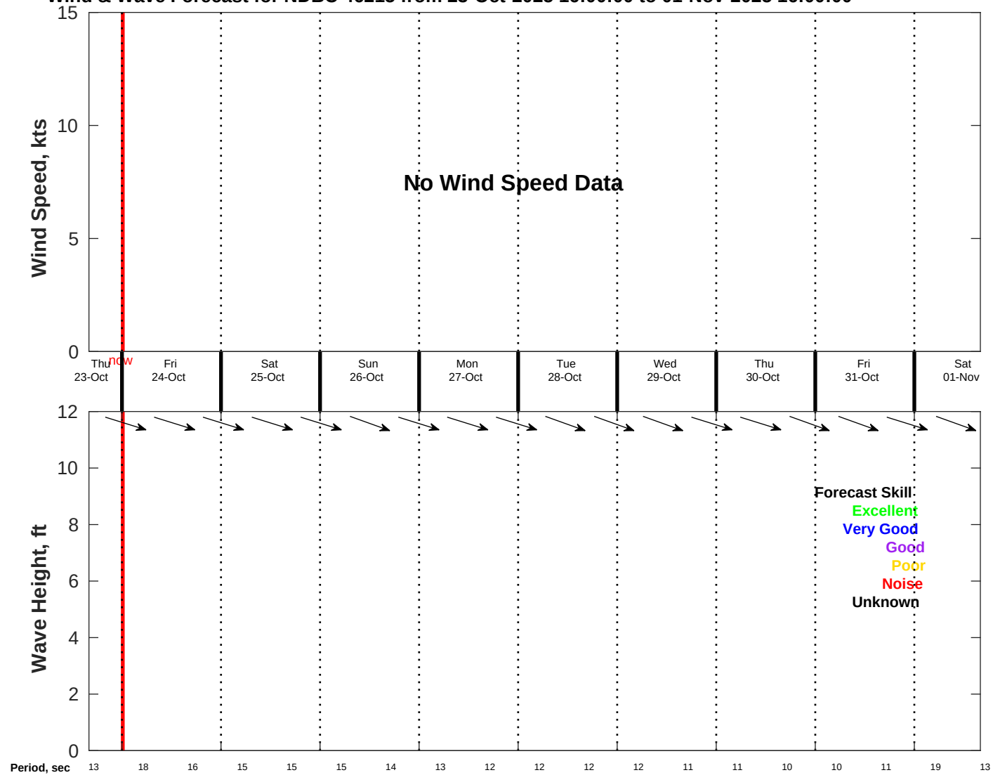
Wind & Wave Forecast for NDBC 46215 from 23-Oct-2025 16:00:00 to 01-Nov-2025 16:00:00
