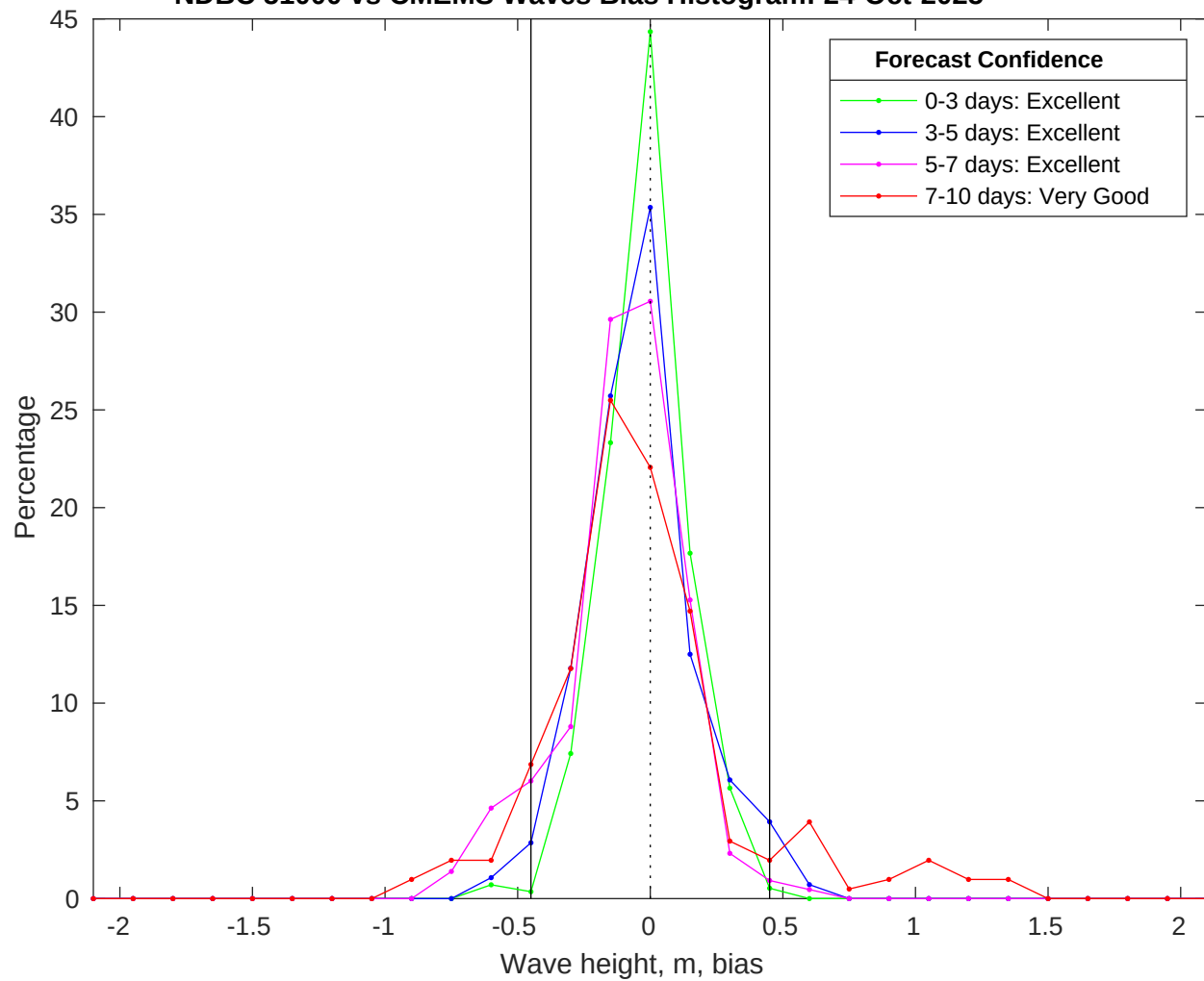
NDBC 51000 vs CMEMS Waves Bias Histogram: 24-Oct-2025
