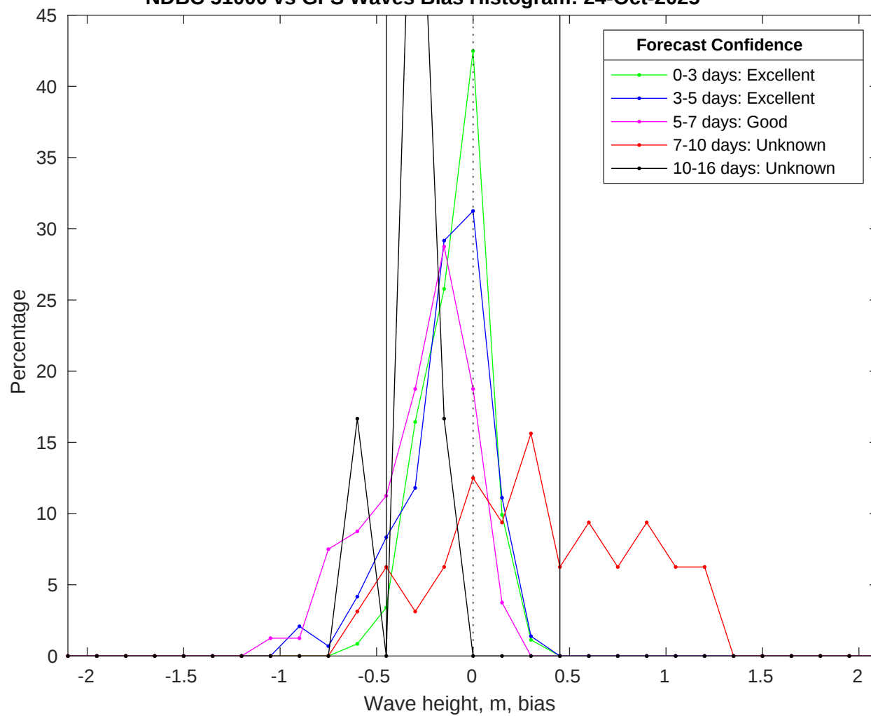
NDBC 51000 vs GFS Waves Bias Histogram: 24-Oct-2025
