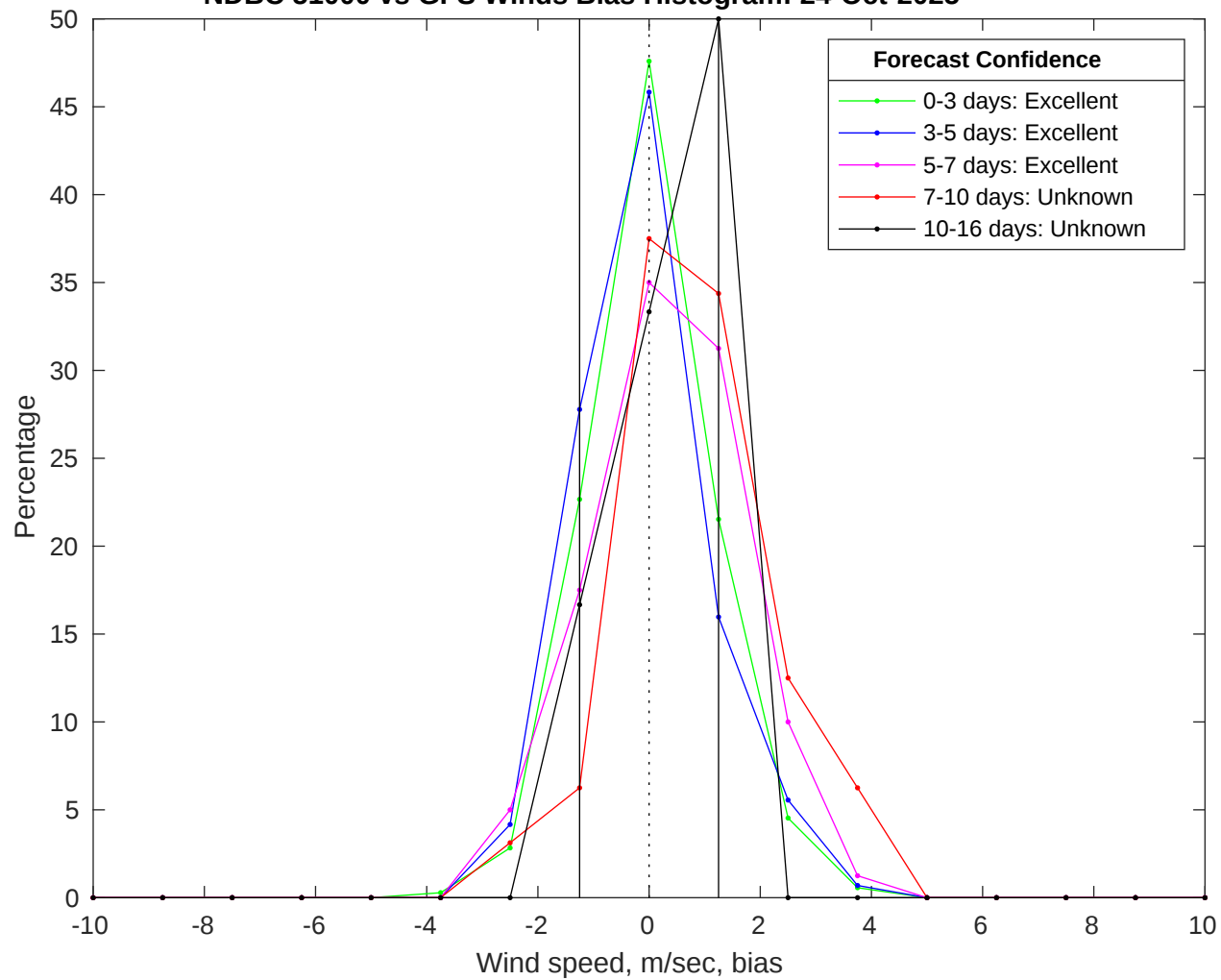
NDBC 51000 vs GFS Winds Bias Histogram: 24-Oct-2025
