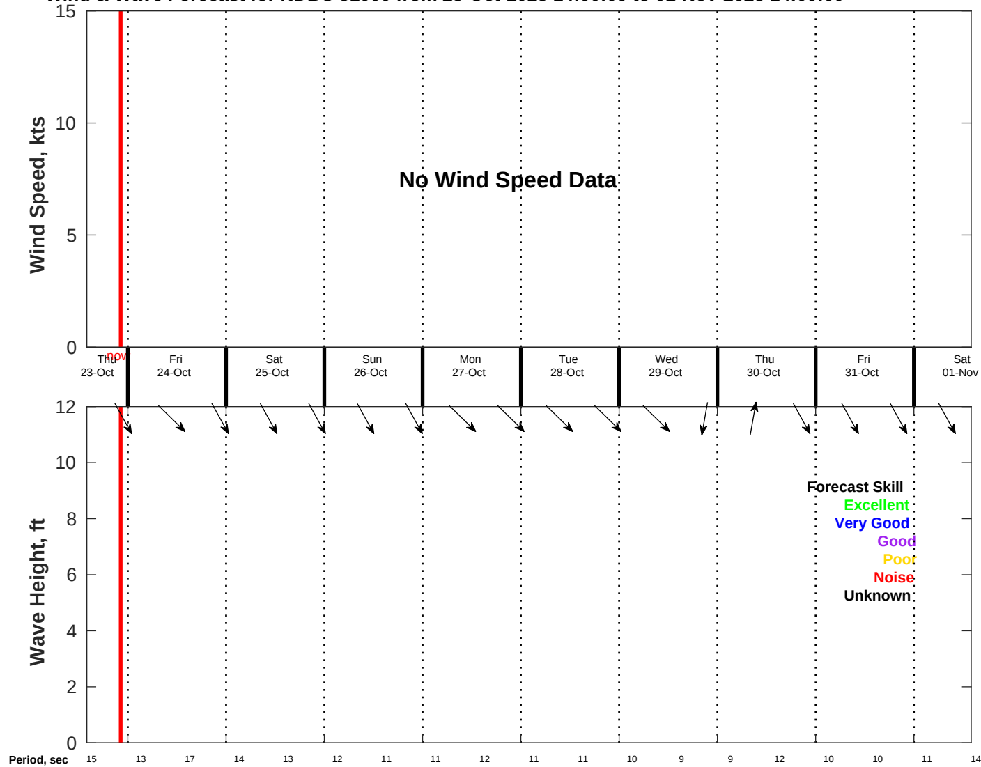
Wind & Wave Forecast for NDBC 51000 from 23-Oct-2025 14:00:00 to 01-Nov-2025 14:00:00
