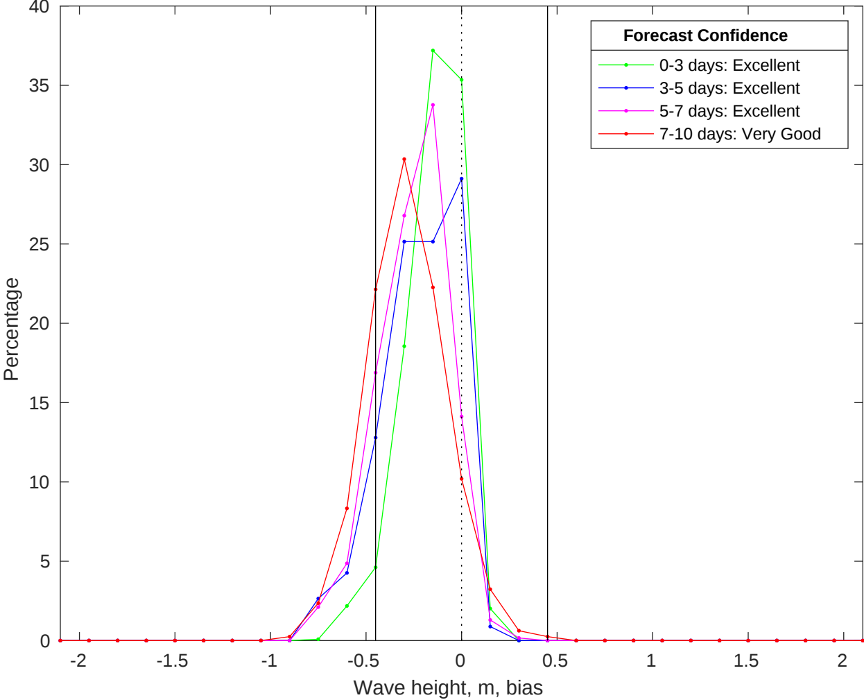
NDBC 52213 vs CMEMS Waves Bias Histogram: 24-Oct-2025
