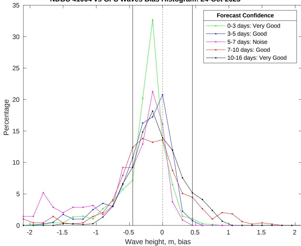
NDBC 41004 vs GFS Waves Bias Histogram: 24-Oct-2025
