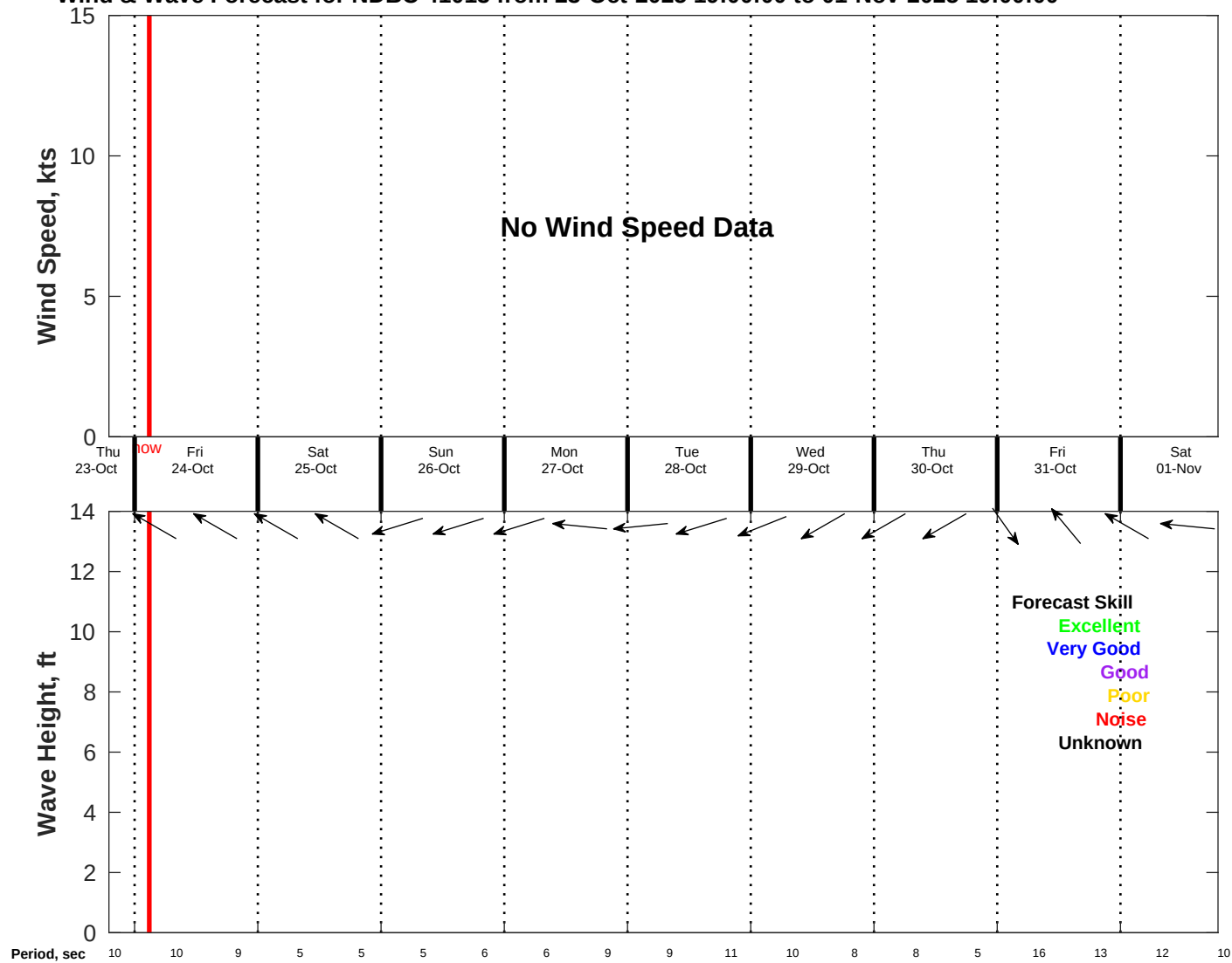
Wind & Wave Forecast for NDBC 41013 from 23-Oct-2025 19:00:00 to 01-Nov-2025 19:00:00
