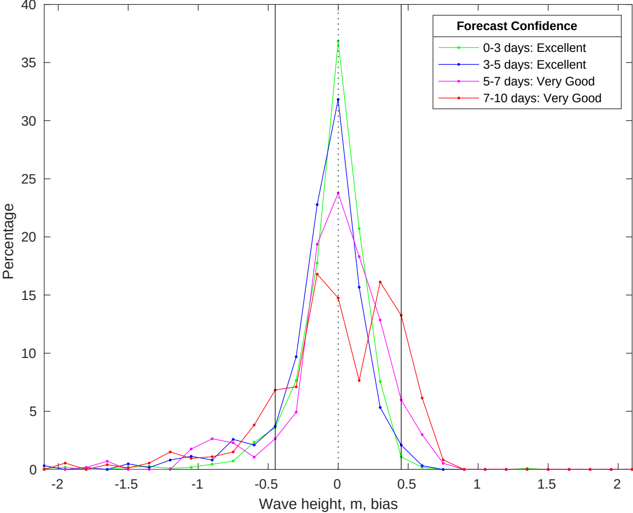
NDBC 41040 vs CMEMS Waves Bias Histogram: 25-Oct-2025
