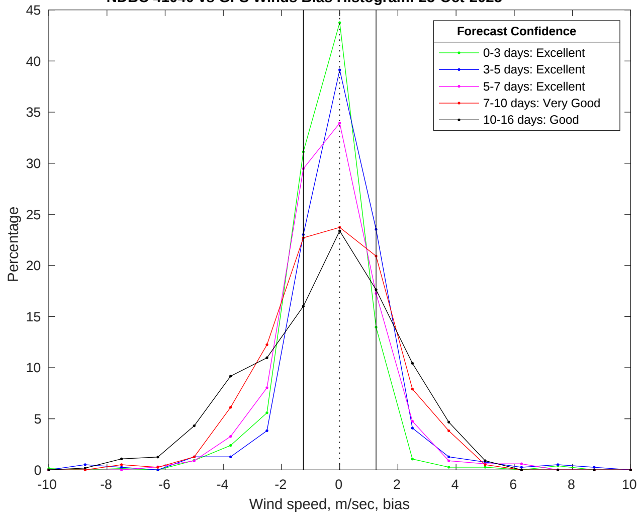
NDBC 41040 vs GFS Winds Bias Histogram: 25-Oct-2025
