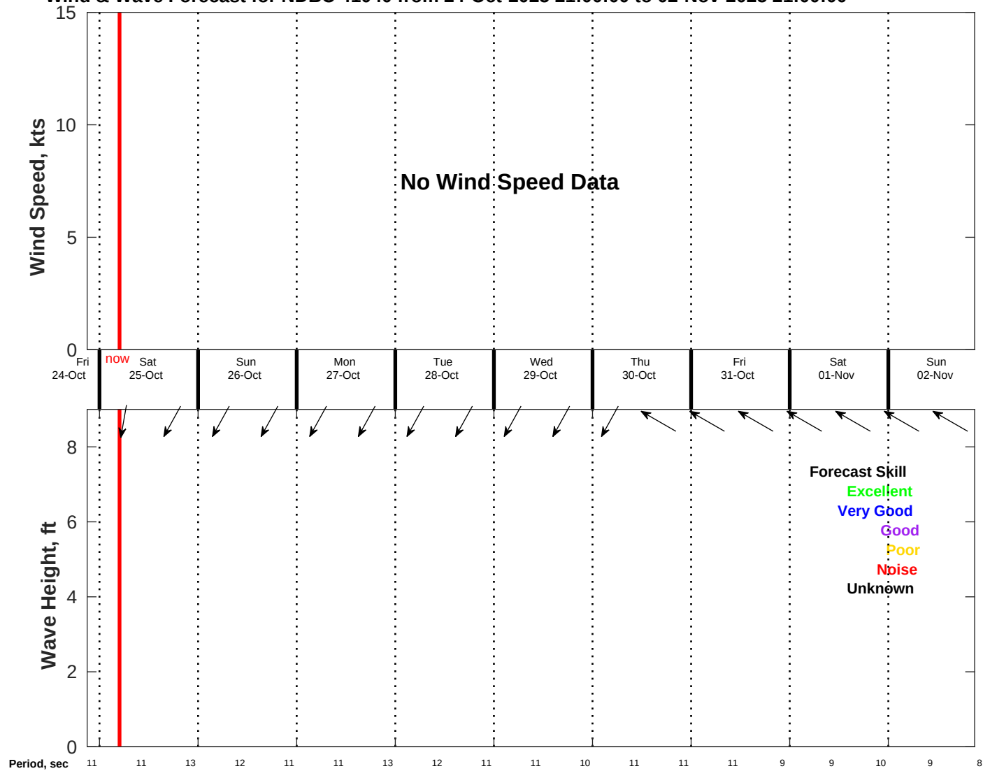
Wind & Wave Forecast for NDBC 41040 from 24-Oct-2025 21:00:00 to 02-Nov-2025 21:00:00
