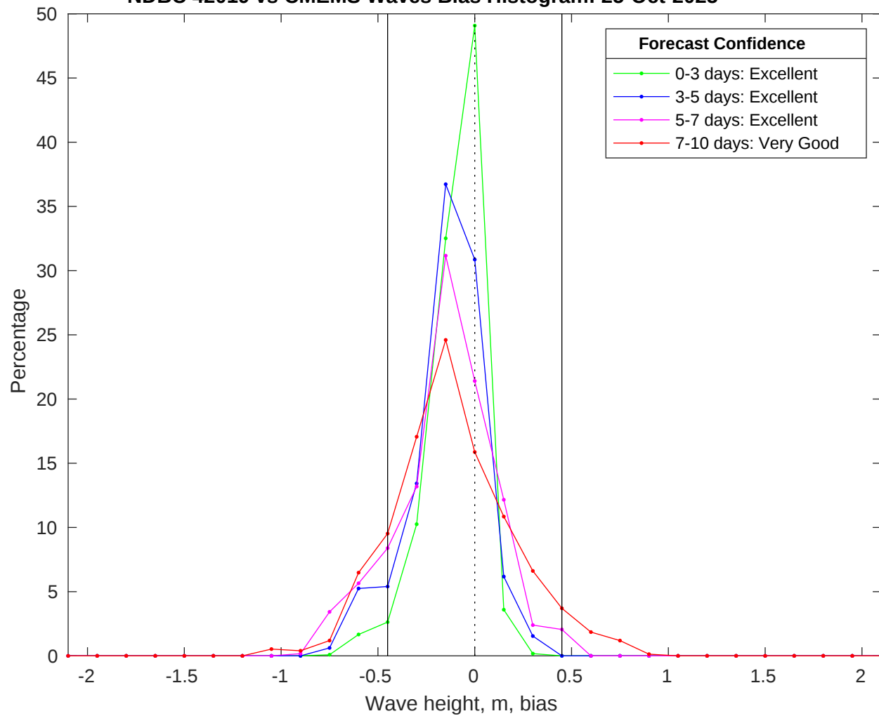
NDBC 42019 vs CMEMS Waves Bias Histogram: 25-Oct-2025
