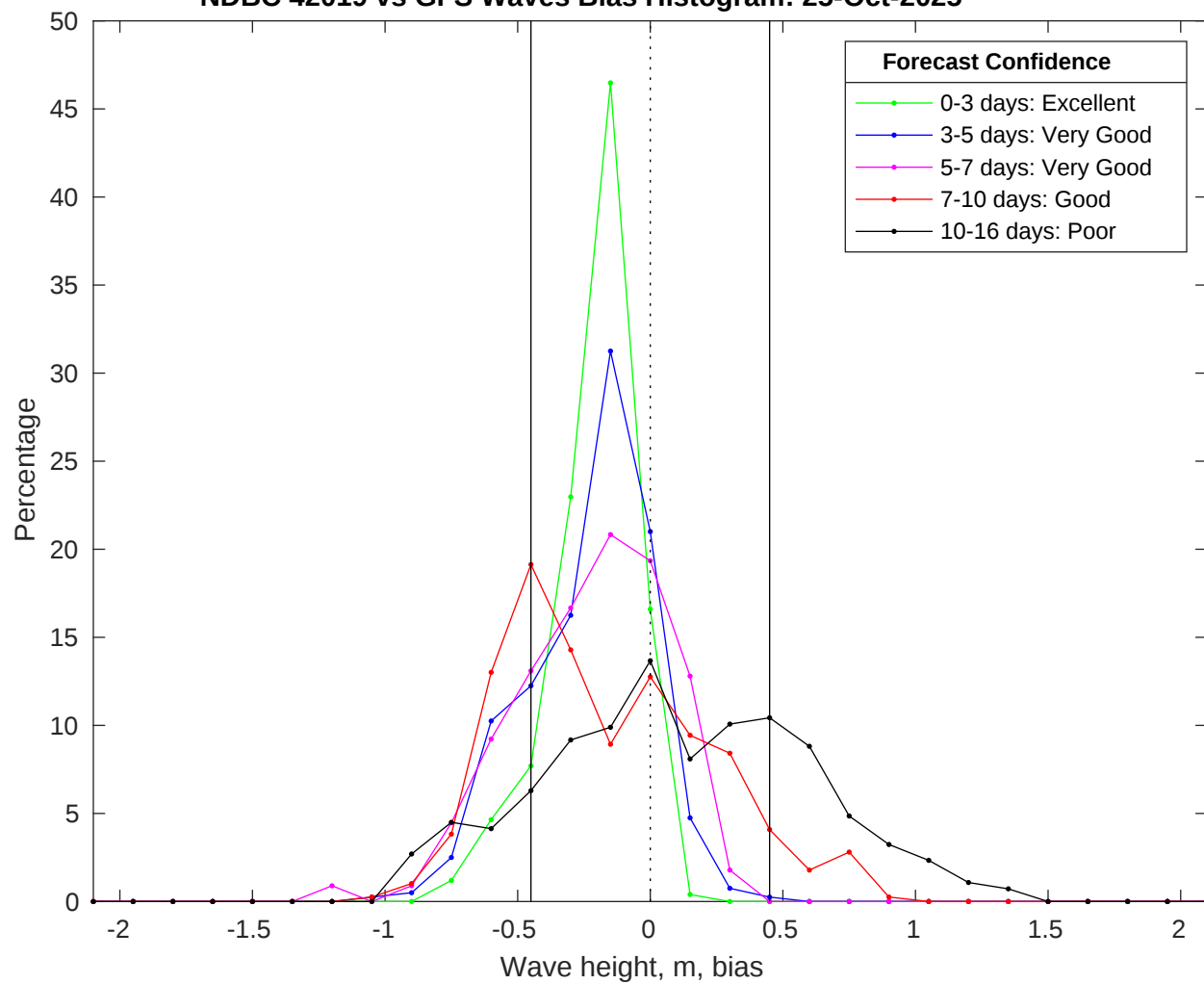
NDBC 42019 vs GFS Waves Bias Histogram: 25-Oct-2025
