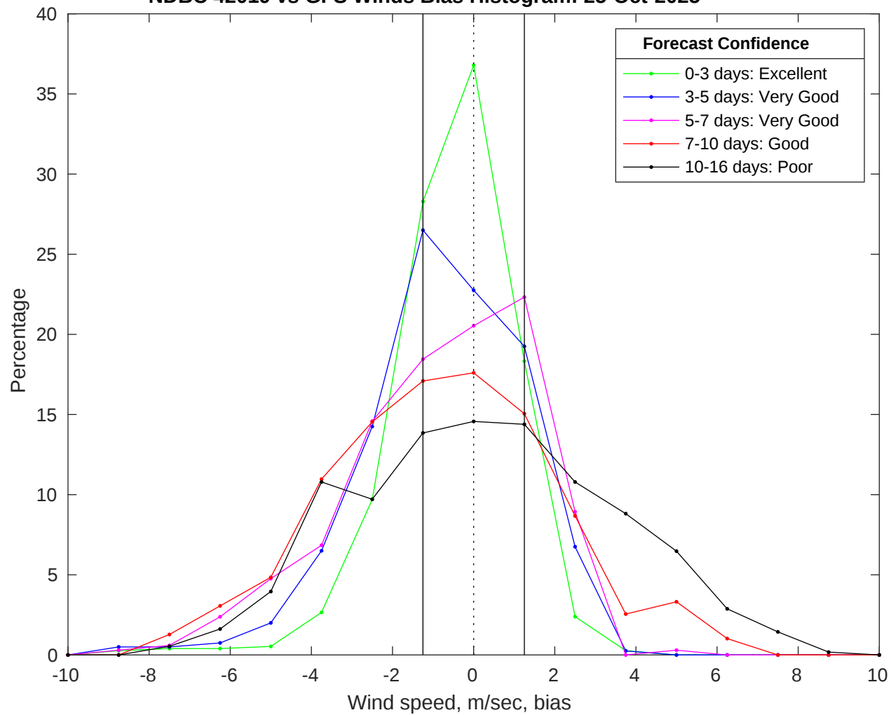
NDBC 42019 vs GFS Winds Bias Histogram: 25-Oct-2025
