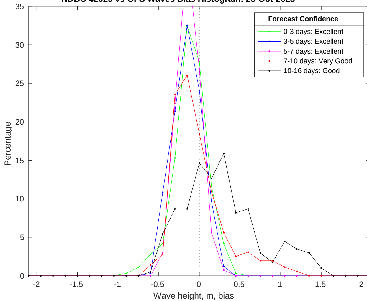
NDBC 42020 vs GFS Waves Bias Histogram: 23-Oct-2025
