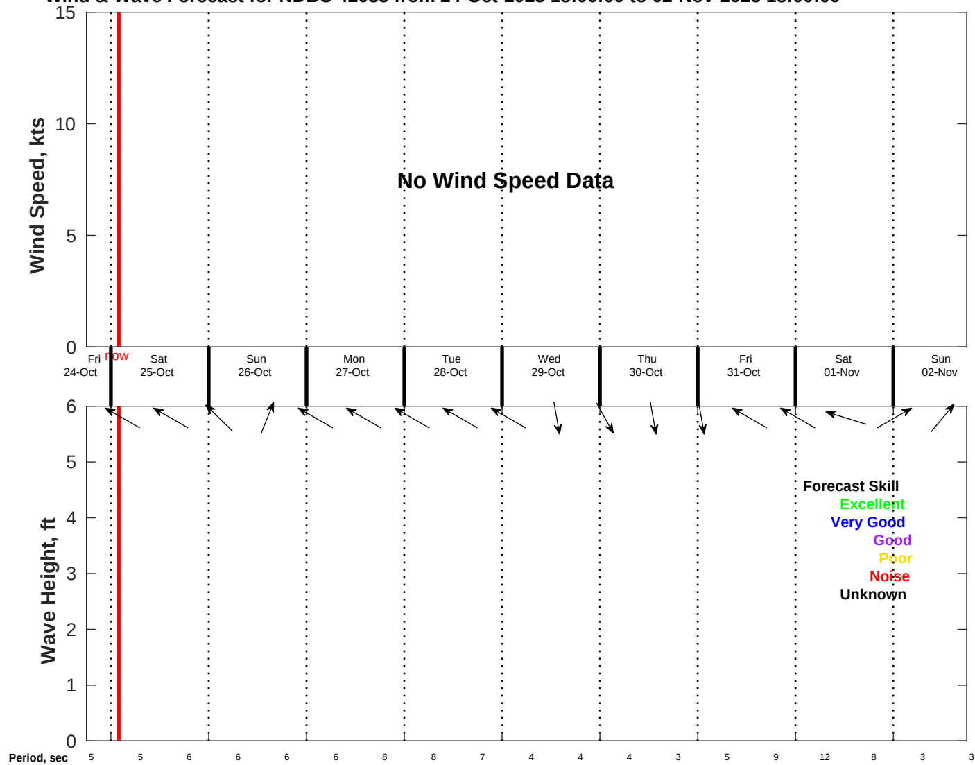
Wind & Wave Forecast for NDBC 42035 from 24-Oct-2025 18:00:00 to 02-Nov-2025 18:00:00
