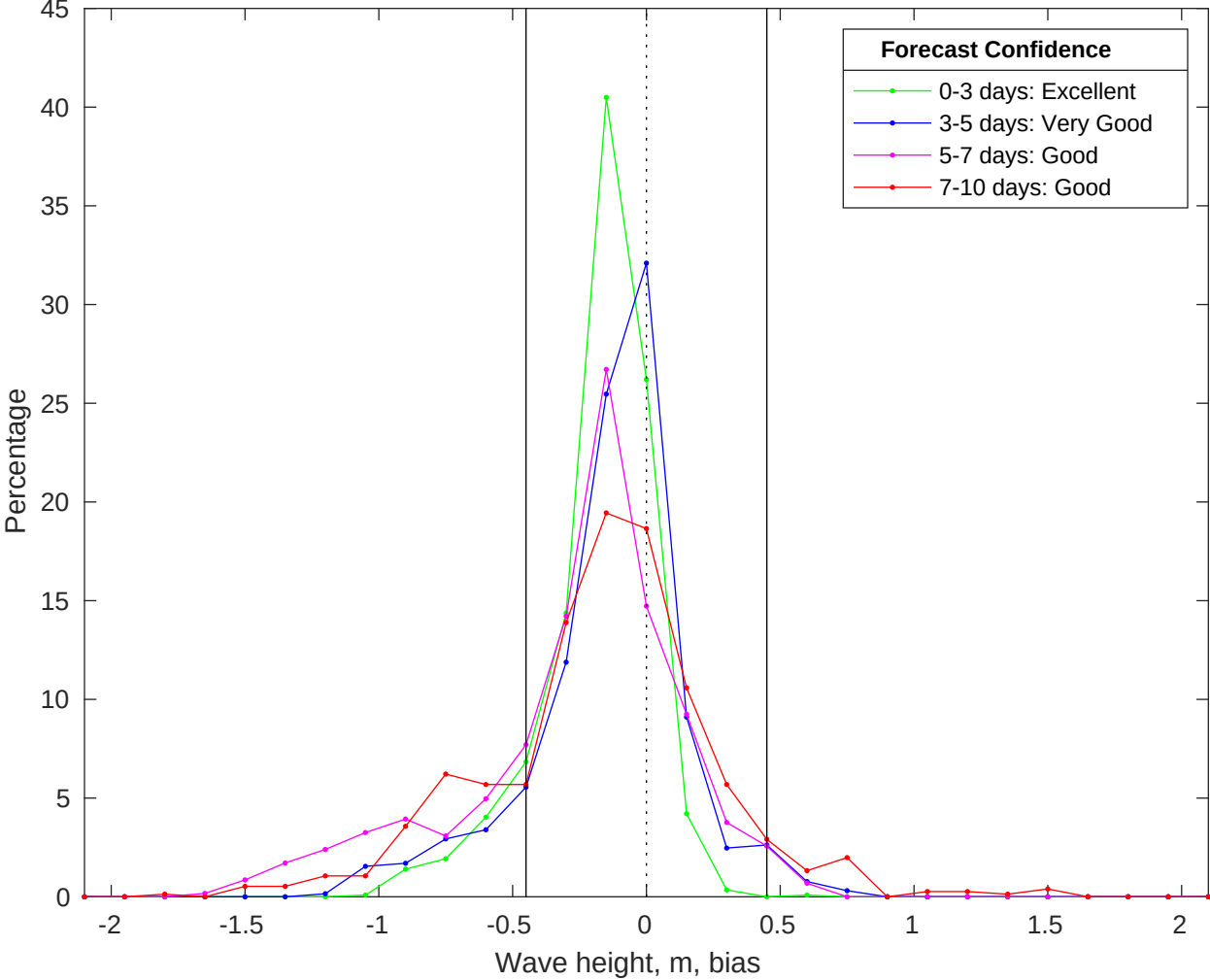
NDBC 42036 vs CMEMS Waves Bias Histogram: 25-Oct-2025
