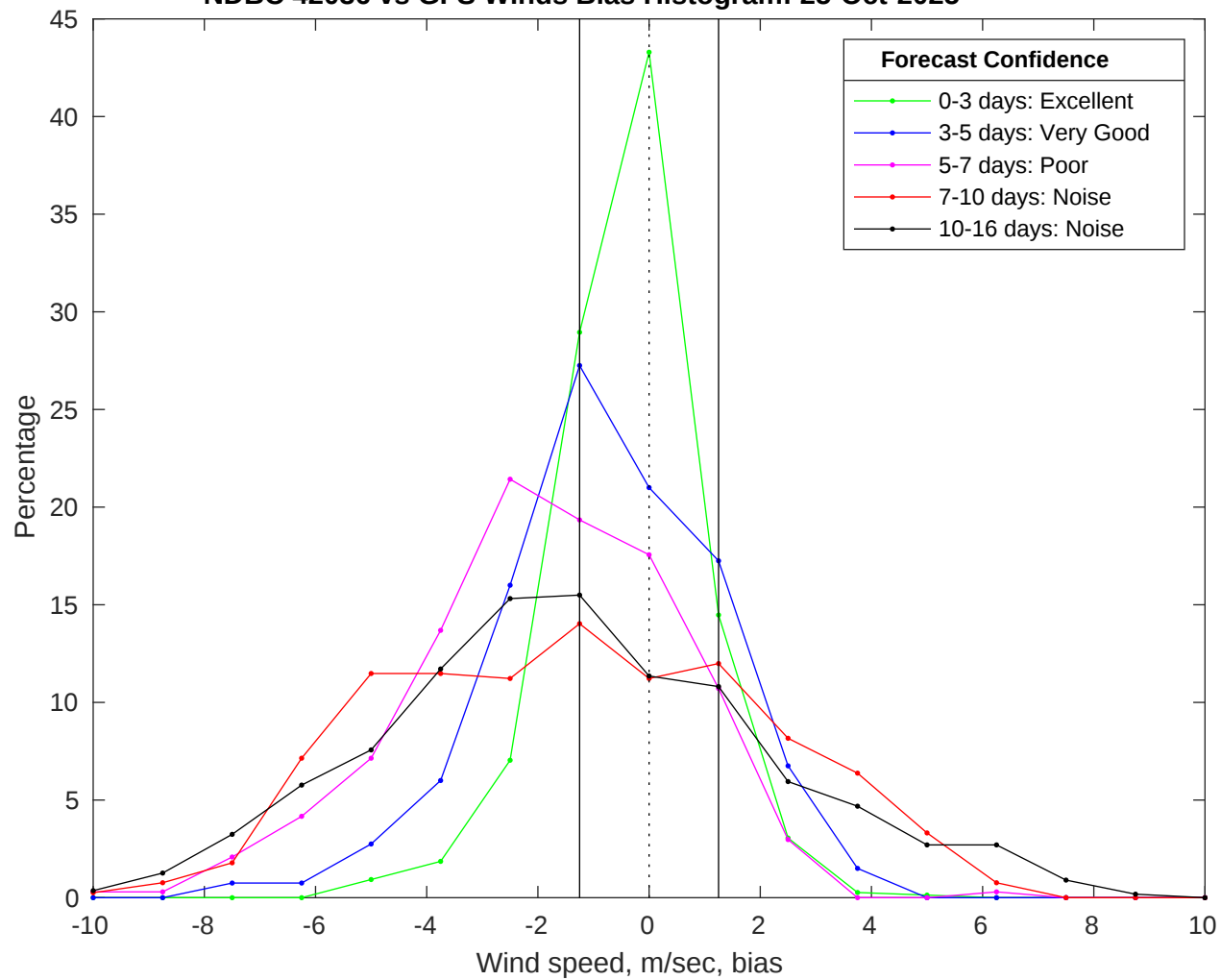
NDBC 42036 vs GFS Winds Bias Histogram: 25-Oct-2025
