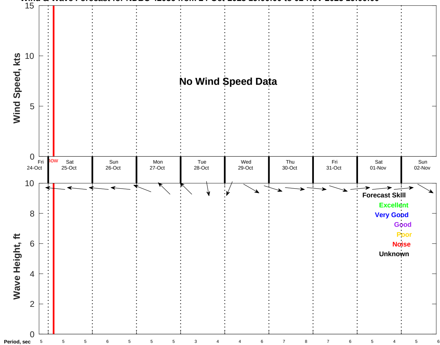
Wind & Wave Forecast for NDBC 42036 from 24-Oct-2025 19:00:00 to 02-Nov-2025 19:00:00
