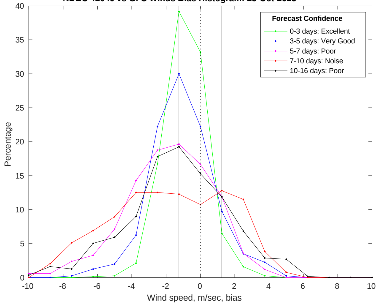
NDBC 42040 vs GFS Winds Bias Histogram: 25-Oct-2025
