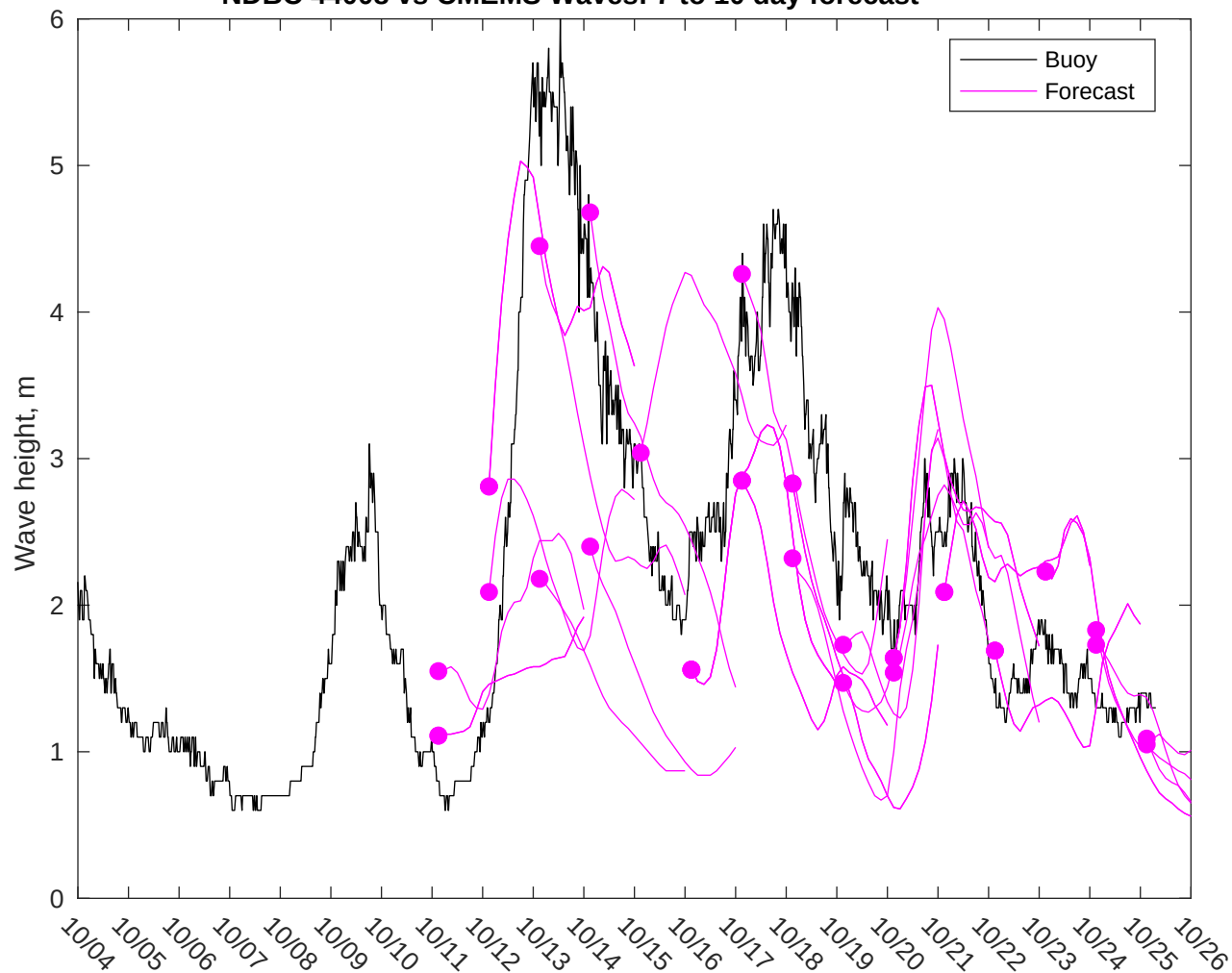
NDBC 44008 vs CMEMS Waves: 7 to 10 day forecast
