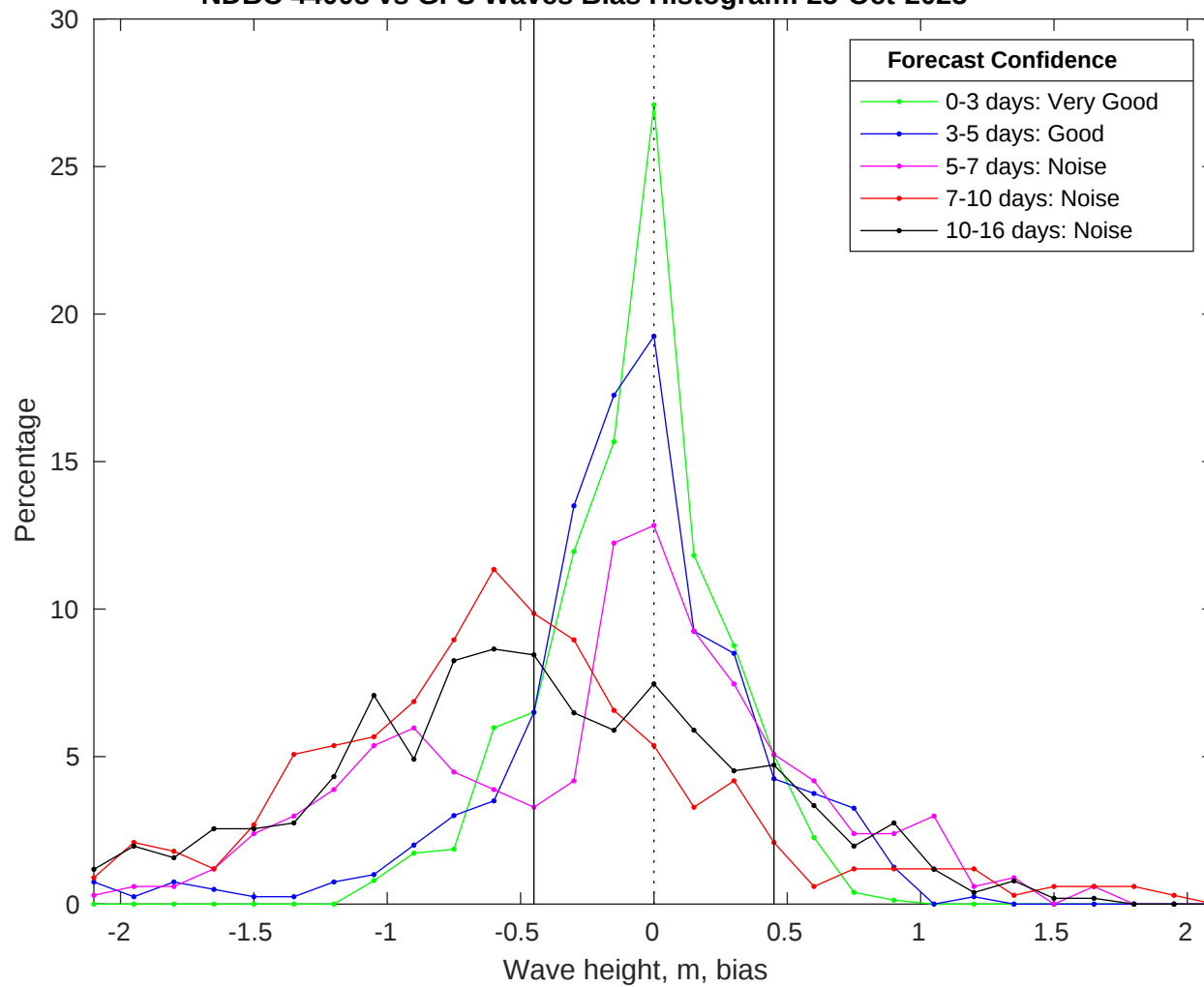
NDBC 44008 vs GFS Waves Bias Histogram: 25-Oct-2025
