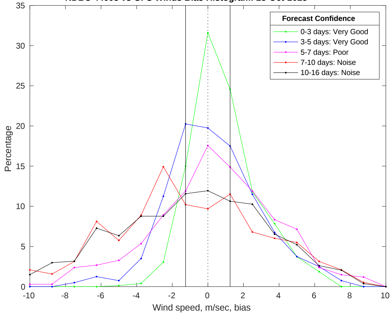
NDBC 44008 vs GFS Winds Bias Histogram: 25-Oct-2025
