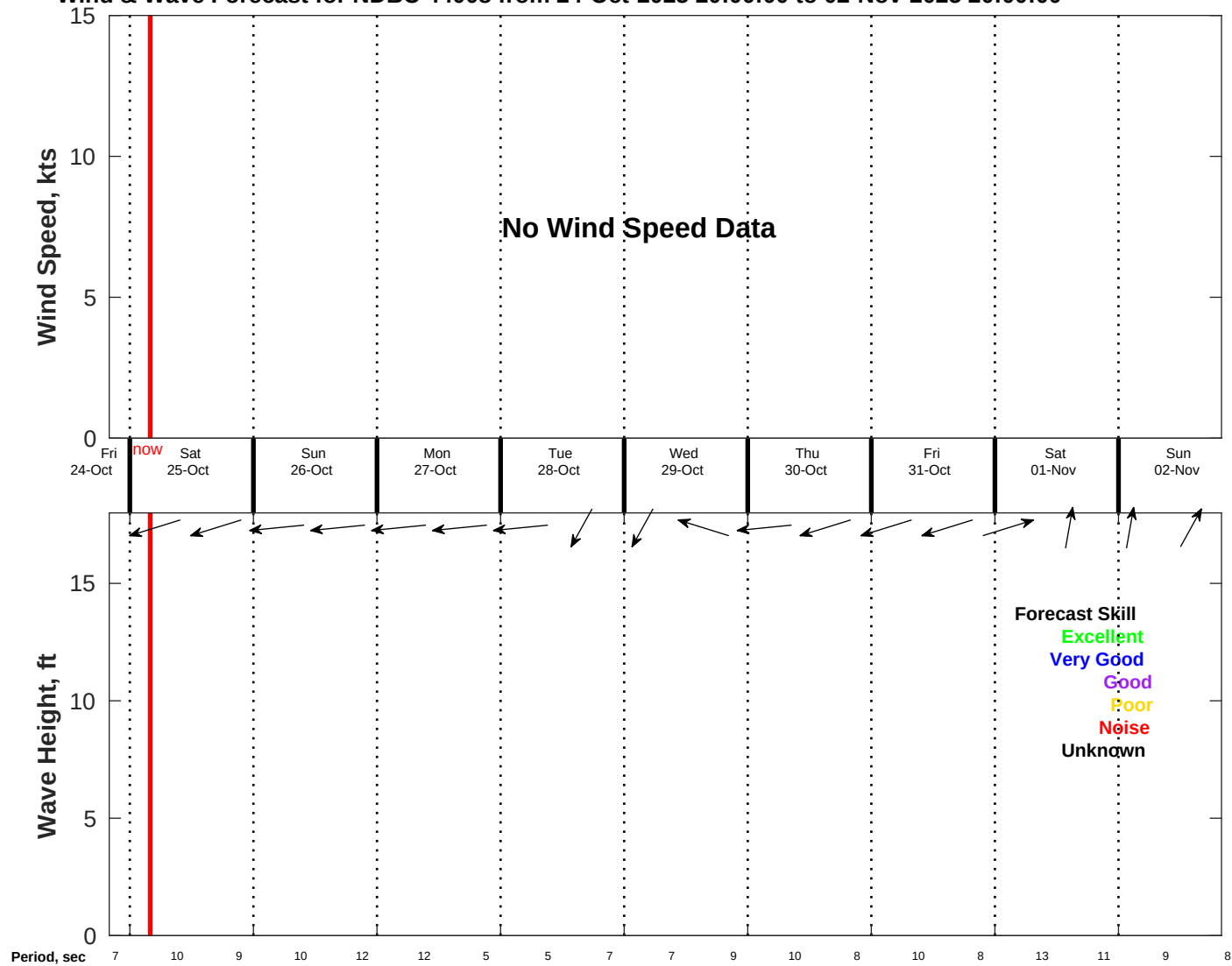
Wind & Wave Forecast for NDBC 44008 from 24-Oct-2025 20:00:00 to 02-Nov-2025 20:00:00
