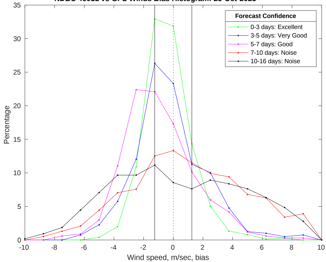
NDBC 46011 vs GFS Winds Bias Histogram: 25-Oct-2025
