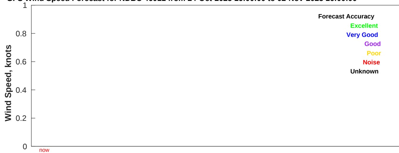
GFS Wind Speed Forecast for NDBC 46011 from 24-Oct-2025 16:00:00 to 02-Nov-2025 16:00:00
