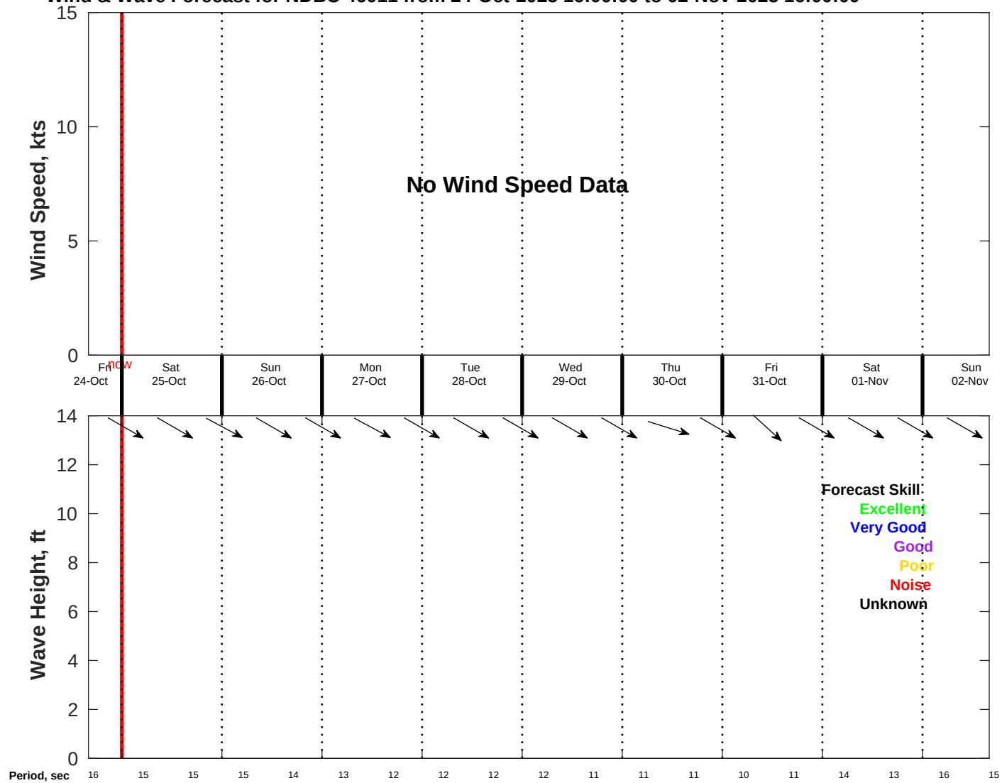
Wind & Wave Forecast for NDBC 46011 from 24-Oct-2025 16:00:00 to 02-Nov-2025 16:00:00
