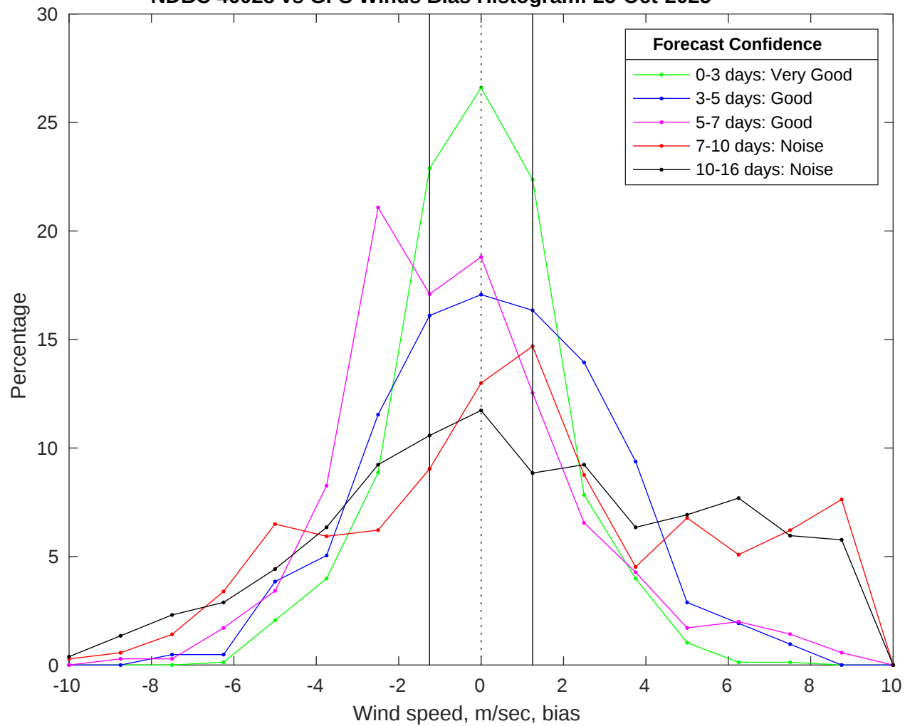
NDBC 46028 vs GFS Winds Bias Histogram: 25-Oct-2025
