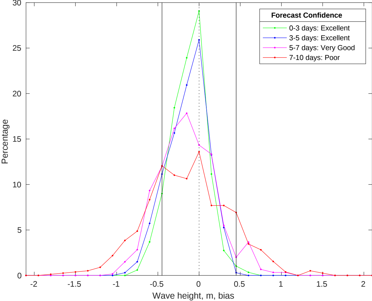
NDBC 46054 vs CMEMS Waves Bias Histogram: 25-Oct-2025
