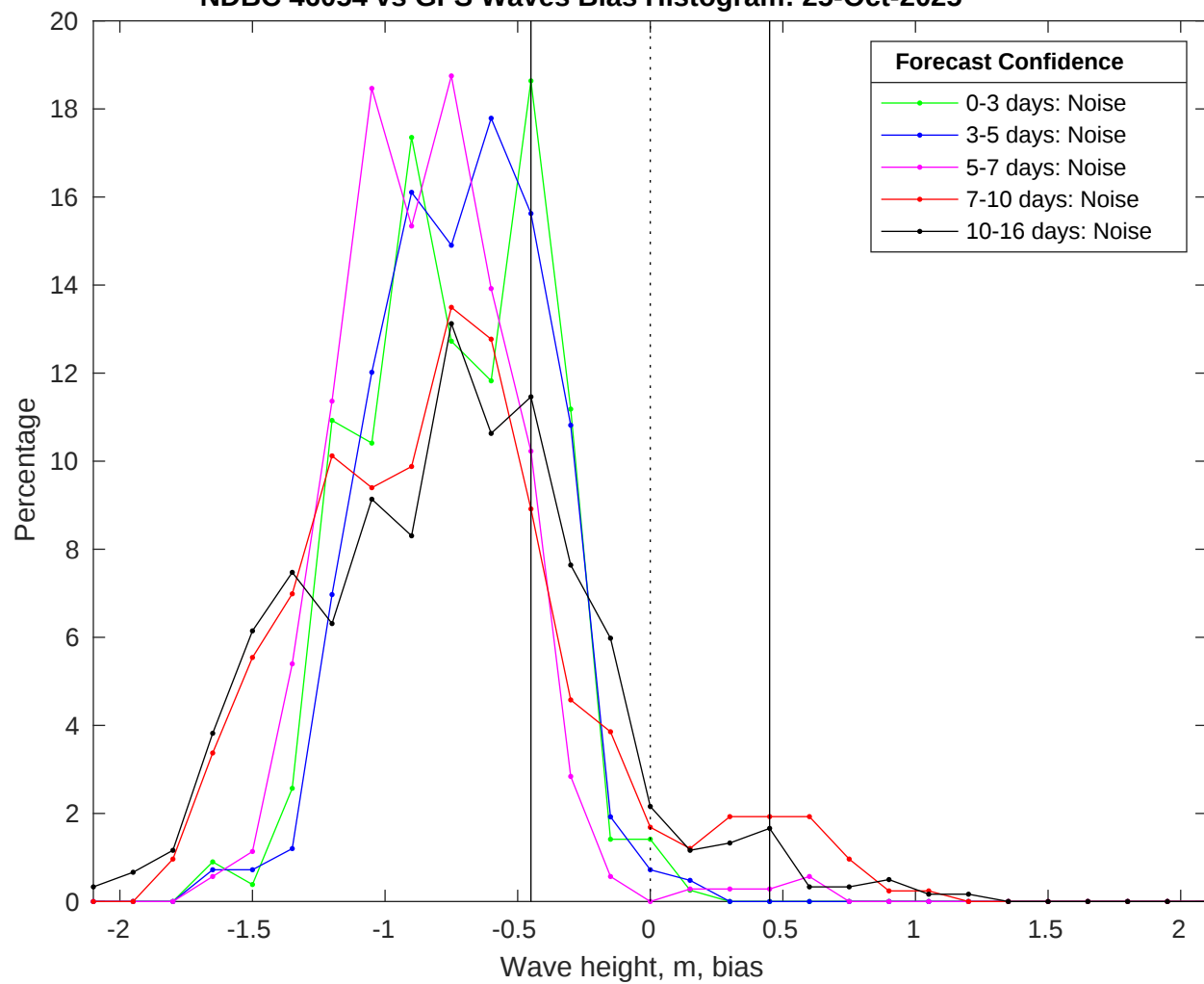
NDBC 46054 vs GFS Waves Bias Histogram: 25-Oct-2025
