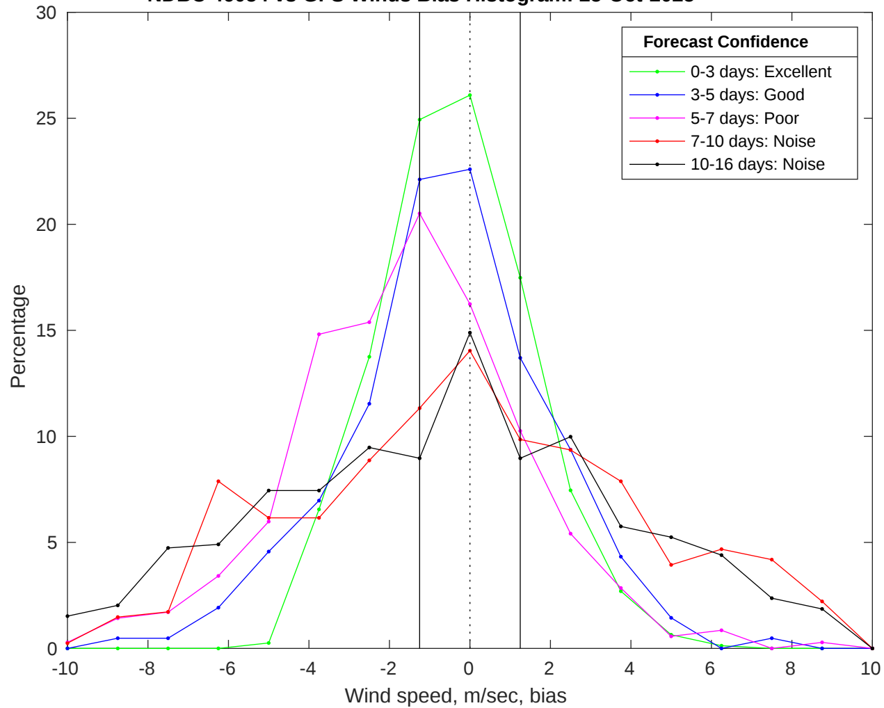
NDBC 46054 vs GFS Winds Bias Histogram: 25-Oct-2025
