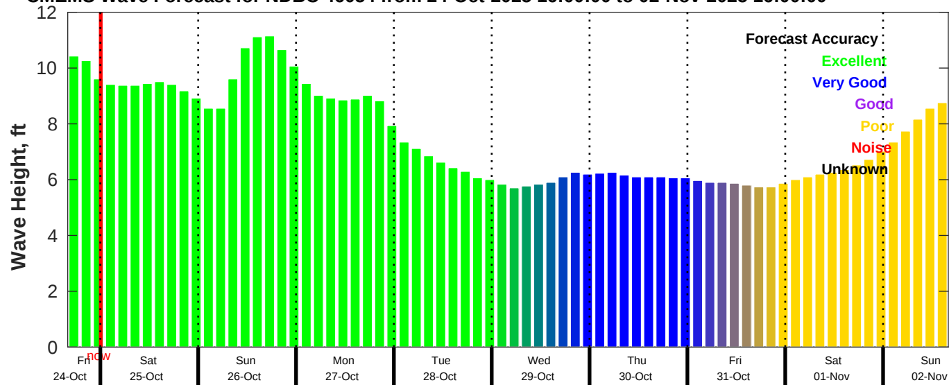
CMEMS Wave Forecast for NDBC 46054 from 24-Oct-2025 16:00:00 to 02-Nov-2025 16:00:00
