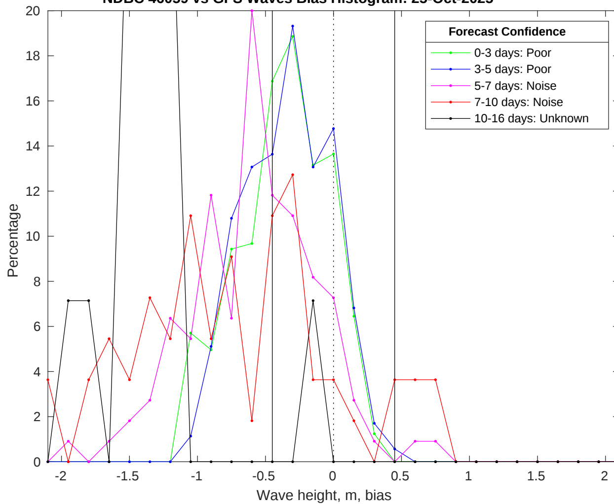
NDBC 46059 vs GFS Waves Bias Histogram: 25-Oct-2025
