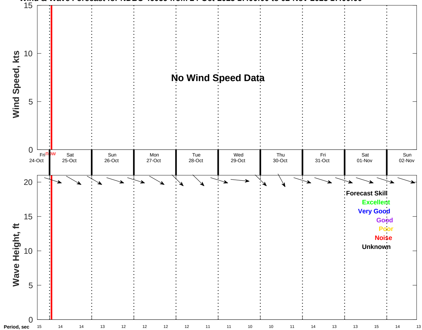
Wind & Wave Forecast for NDBC 46059 from 24-Oct-2025 17:00:00 to 02-Nov-2025 17:00:00
