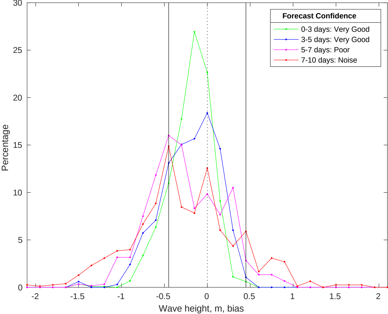
NDBC 46069 vs CMEMS Waves Bias Histogram: 25-Oct-2025
