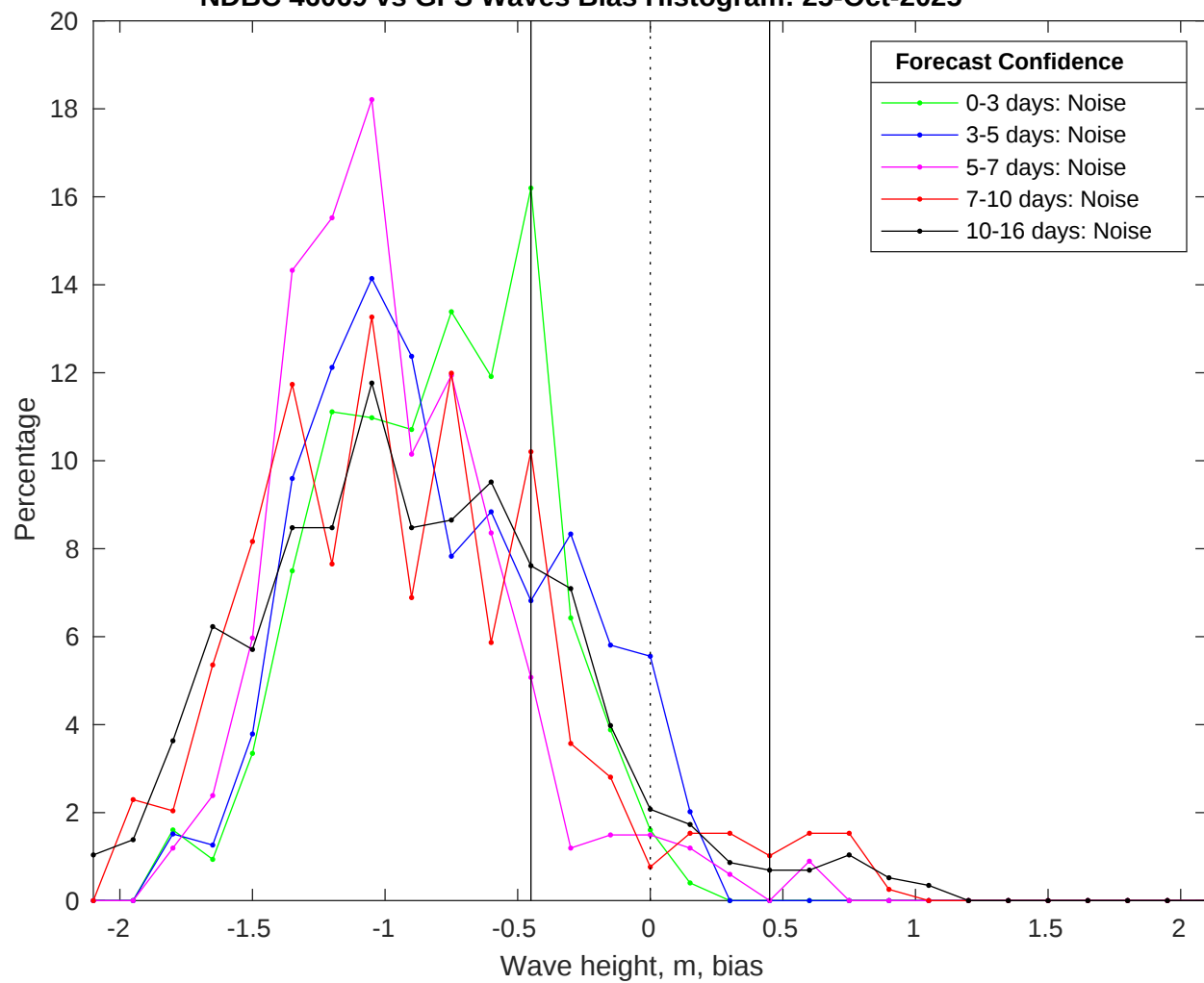
NDBC 46069 vs GFS Waves Bias Histogram: 25-Oct-2025
