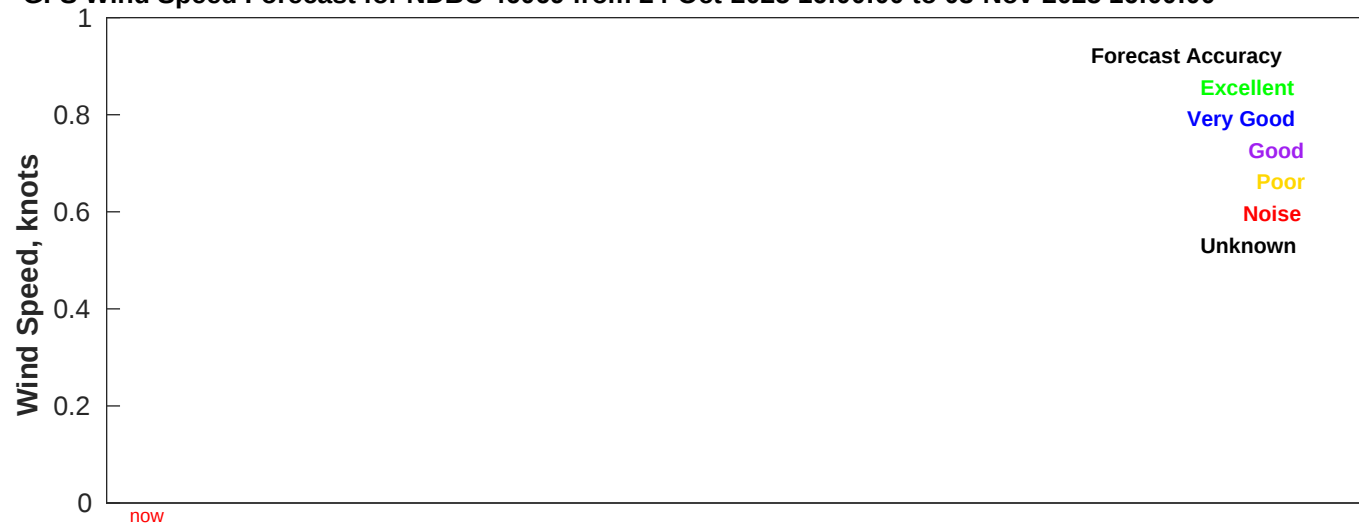
GFS Wind Speed Forecast for NDBC 46069 from 24-Oct-2025 16:00:00 to 03-Nov-2025 16:00:00
