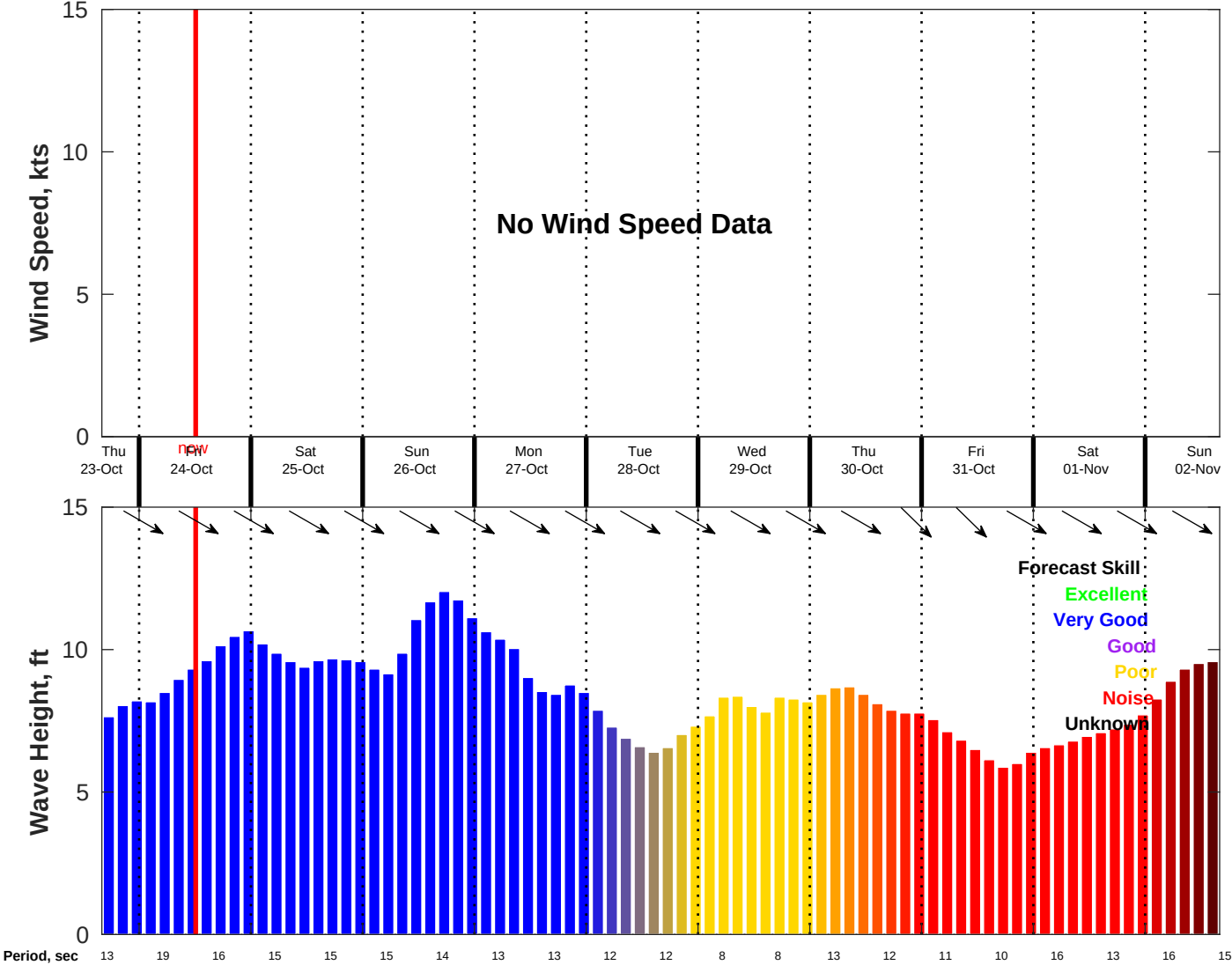
Wind & Wave Forecast for NDBC 46069 from 23-Oct-2025 16:00:00 to 02-Nov-2025 16:00:00
