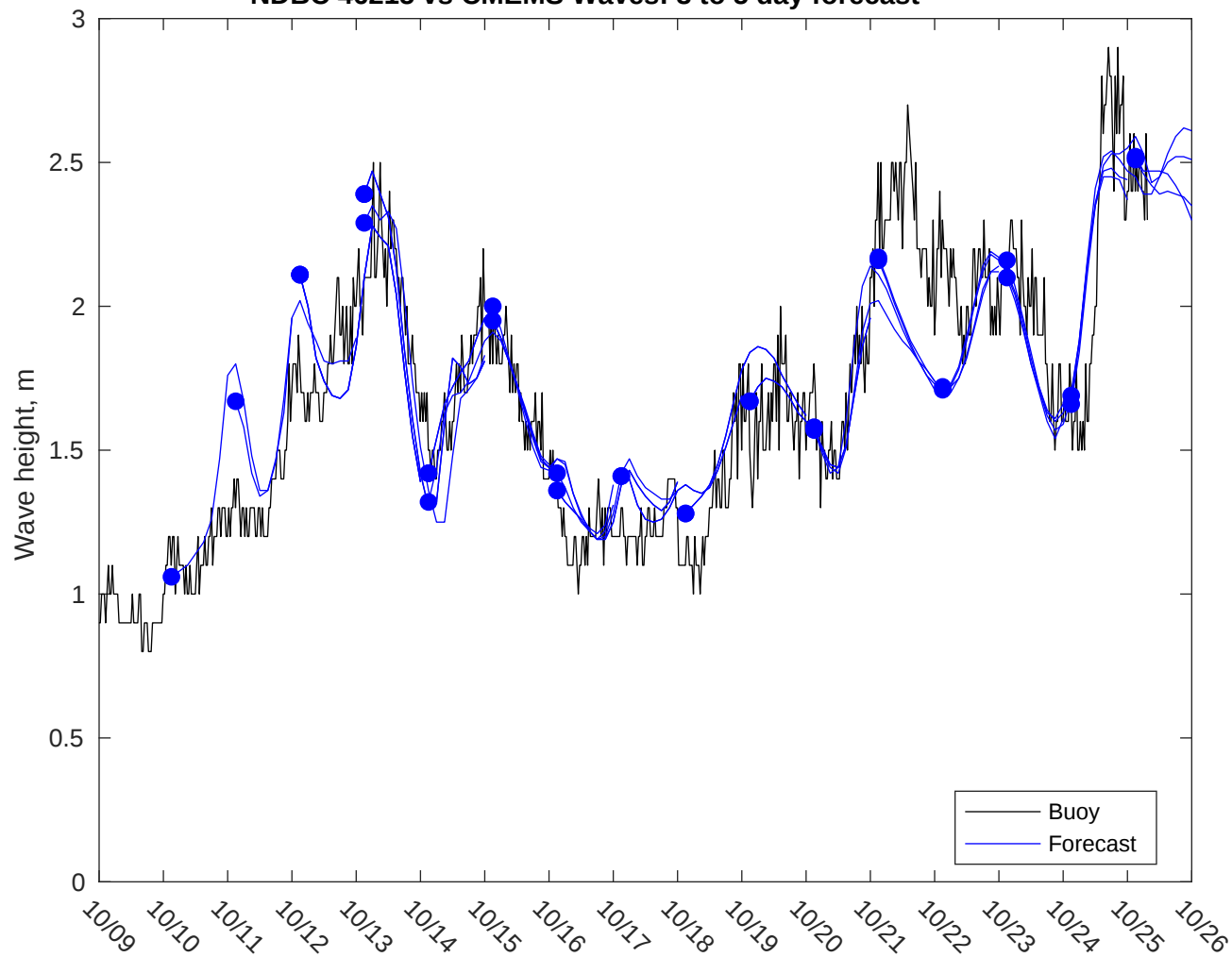
NDBC 46215 vs CMEMS Waves: 3 to 5 day forecast
