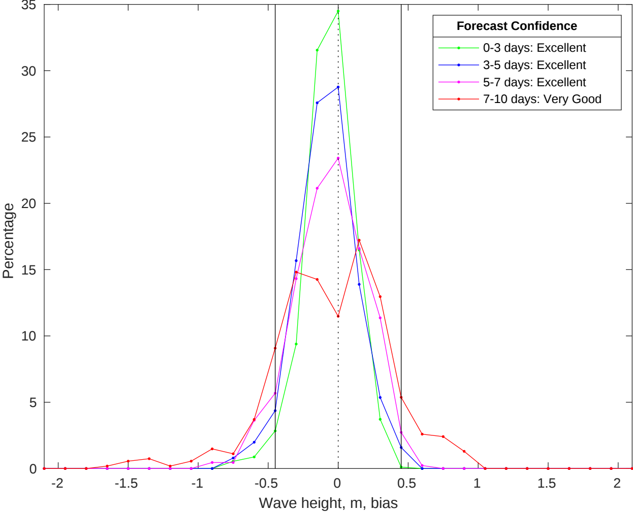
NDBC 46215 vs CMEMS Waves Bias Histogram: 25-Oct-2025
