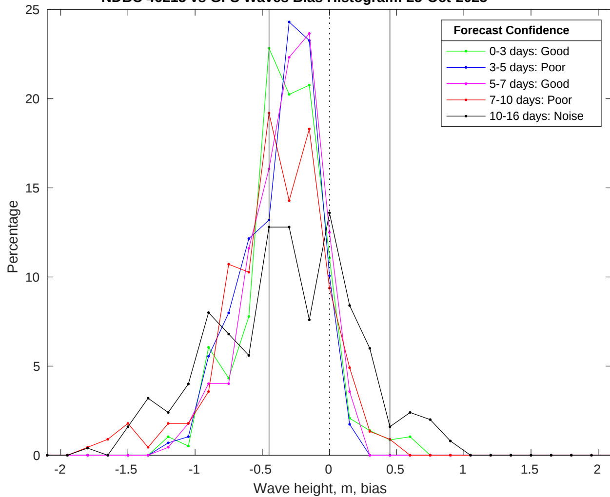
NDBC 46215 vs GFS Waves Bias Histogram: 25-Oct-2025
