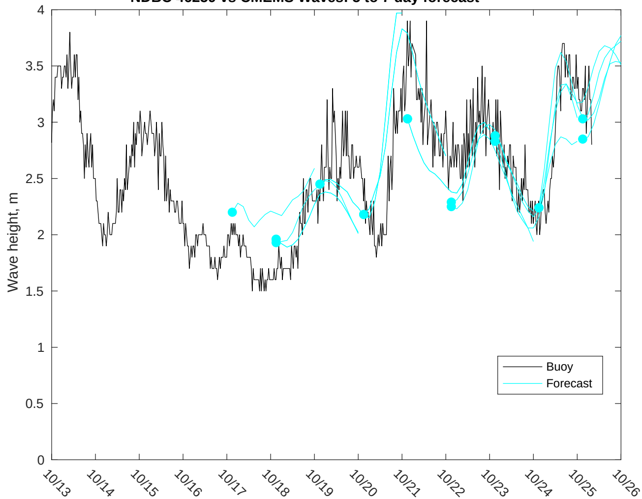
NDBC 46259 vs CMEMS Waves: 5 to 7 day forecast
