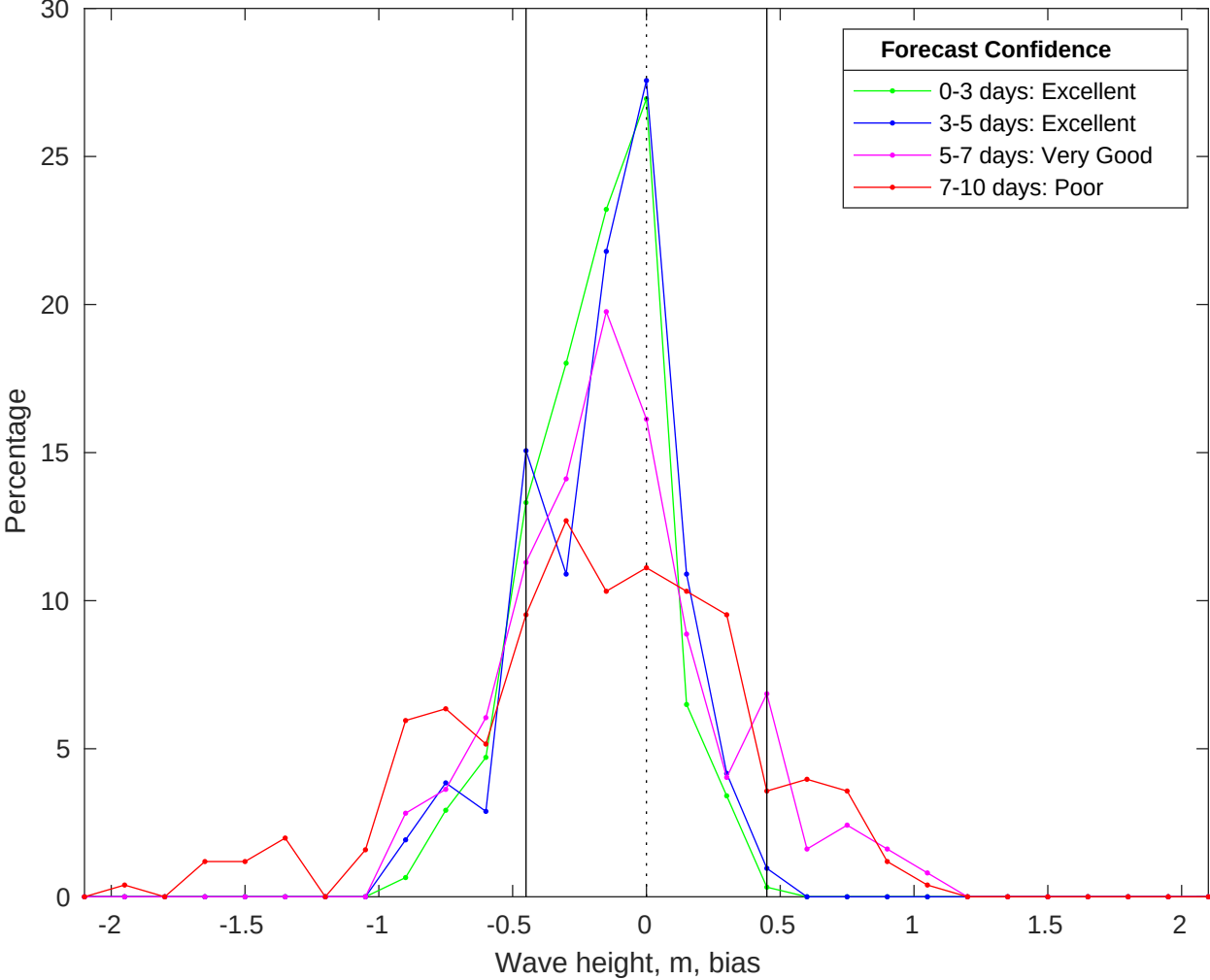
NDBC 46259 vs CMEMS Waves Bias Histogram: 25-Oct-2025
