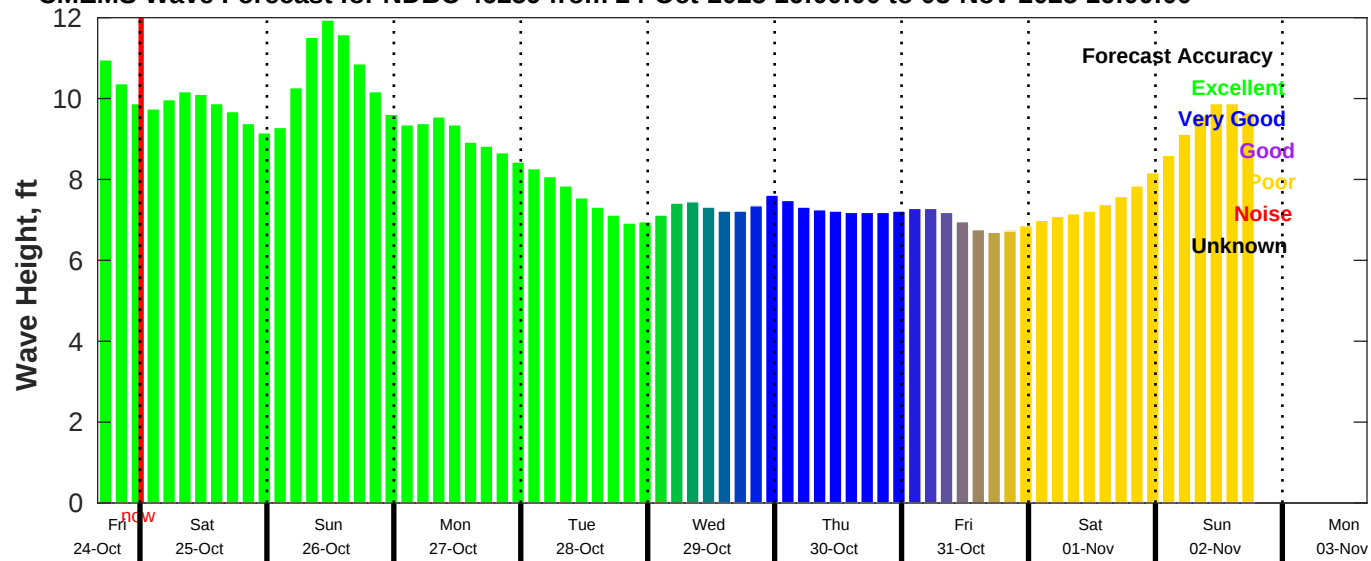
CMEMS Wave Forecast for NDBC 46259 from 24-Oct-2025 16:00:00 to 03-Nov-2025 16:00:00
