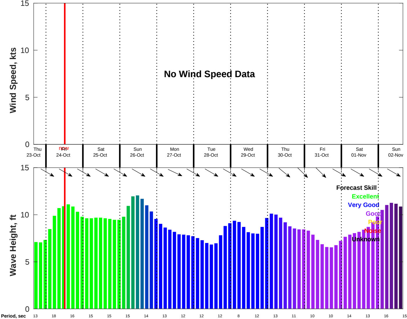
Wind & Wave Forecast for NDBC 46259 from 23-Oct-2025 16:00:00 to 02-Nov-2025 16:00:00
