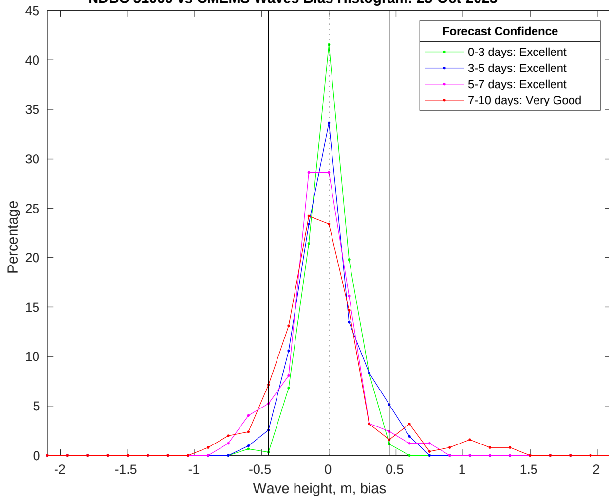
NDBC 51000 vs CMEMS Waves Bias Histogram: 25-Oct-2025
