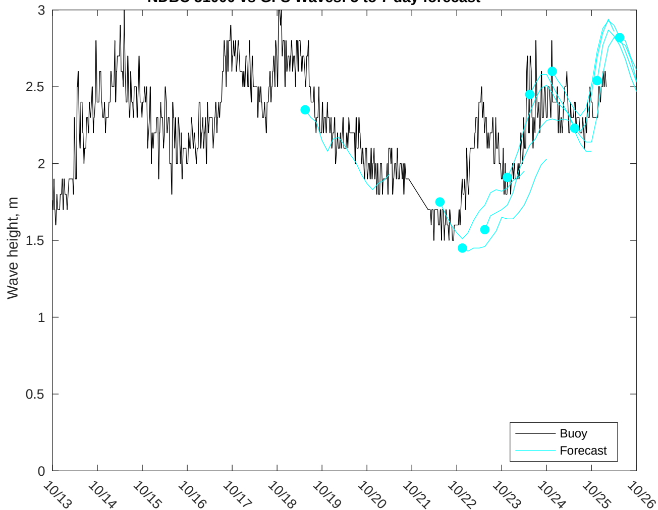
NDBC 51000 vs GFS Waves: 5 to 7 day forecast
